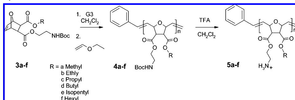
Scheme 2. Polymer Synthesis a
