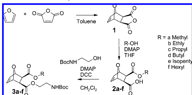
Scheme 1. Monomer Synthesis a
